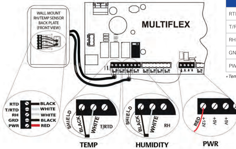
Sensor and Input Board Wiring
