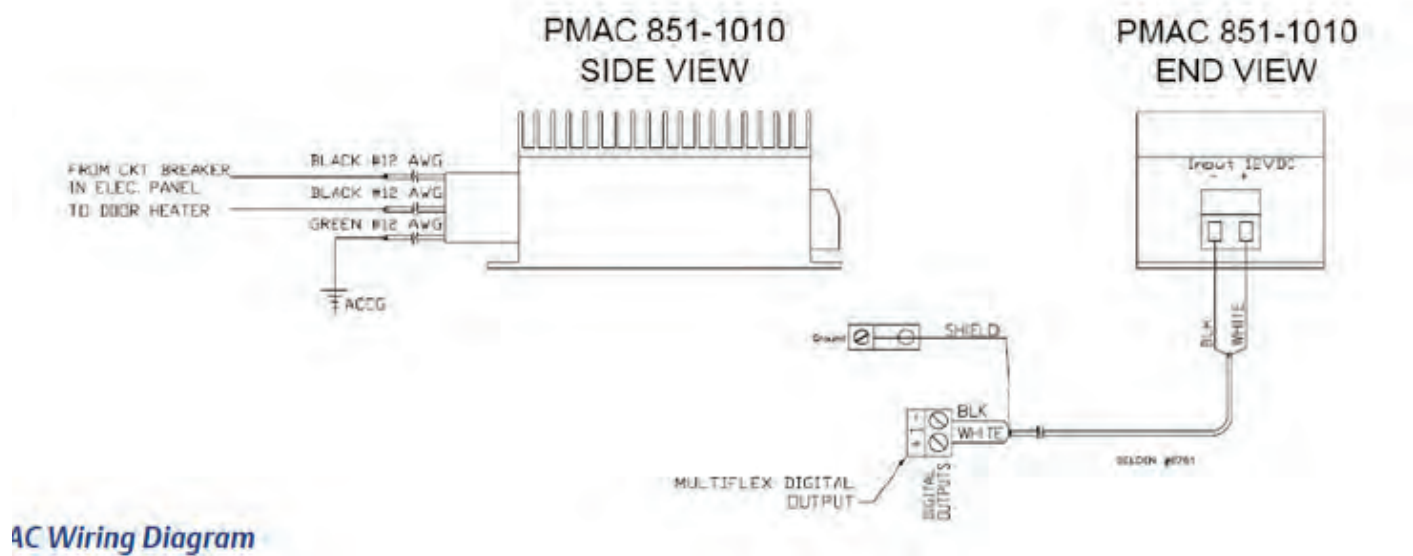
PMAC Wiring Diagram
