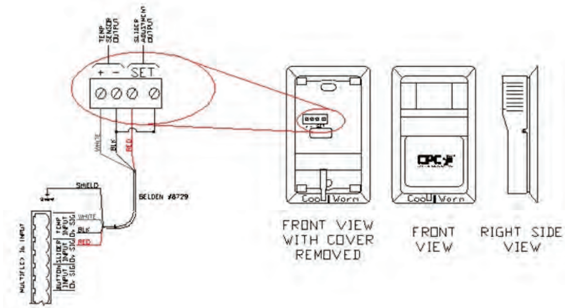
Sensor Wiring Diagram
