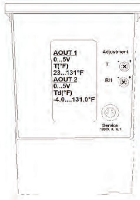
Dewpoint Sensor
