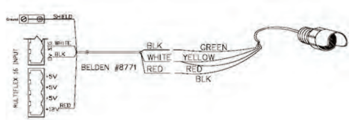
Sensor Wiring Diagram
