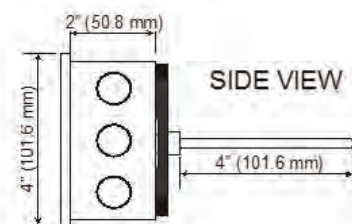
Temperature Sensor Dimensions
