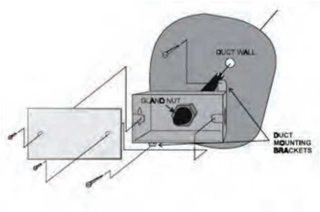
Humidity Sensor Exploded View
