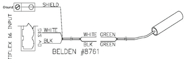
Sensor Wiring Diagram
