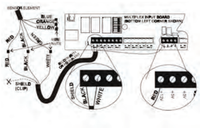
Sensor and Input Board Wiring
