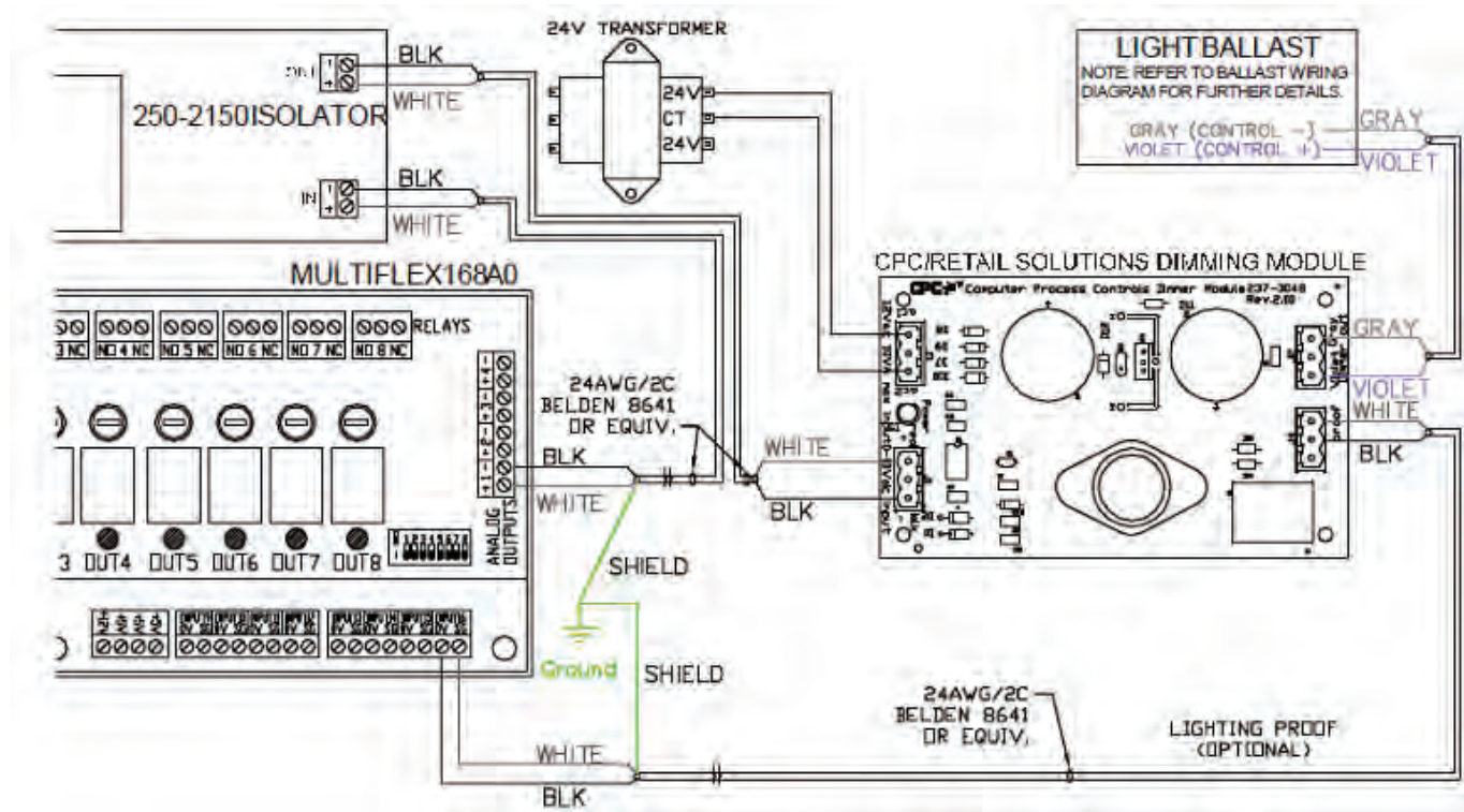
Typical Light Dimming Module Wiring Diagram
