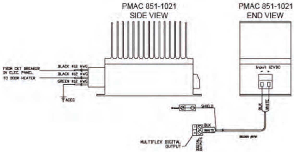
PMAC Wiring Diagram
