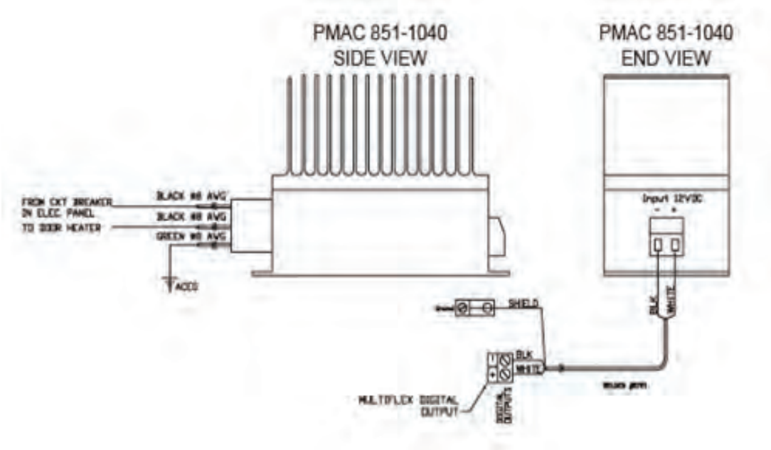
PMAC Wiring Diagram
