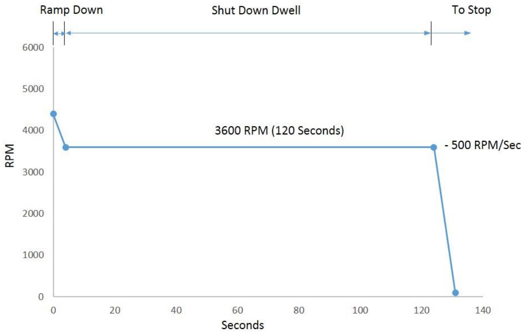
Figure 10 Shut Down Procedure
