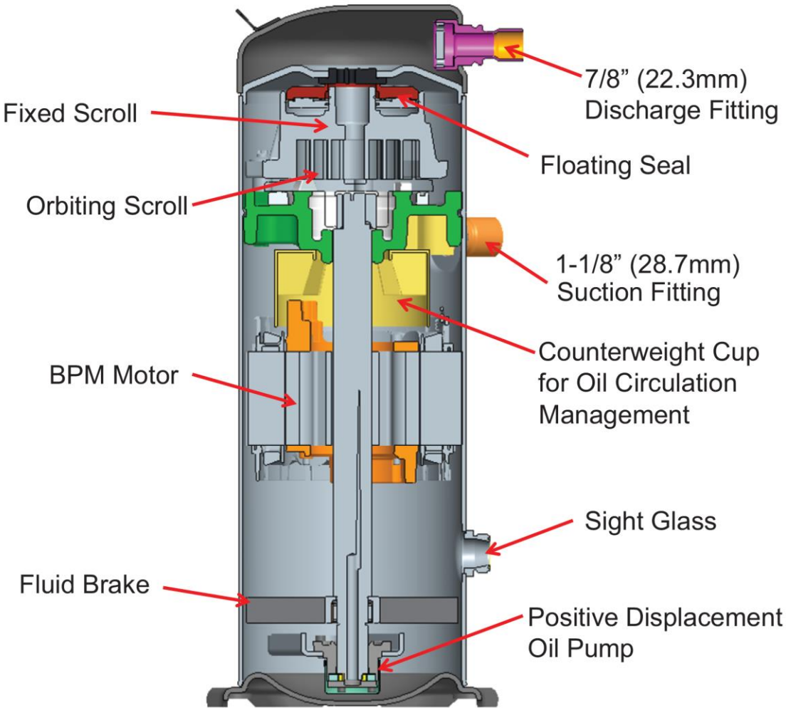
Figure 7 ZPV066 and ZPV096 Cross Sectional View
