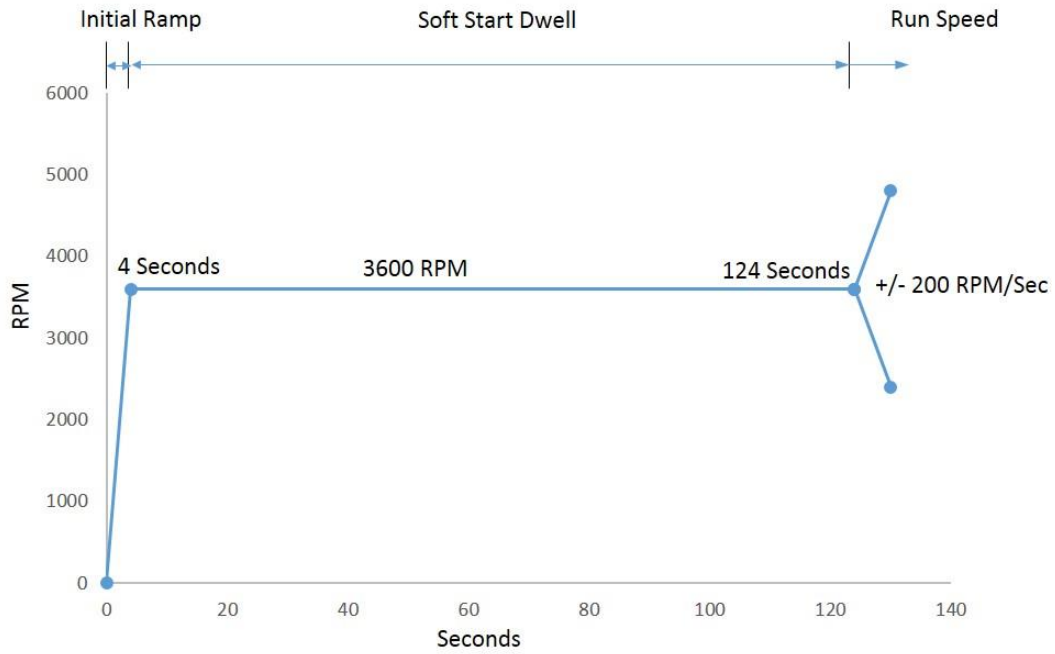
Figure 9 Start Up Procedure
