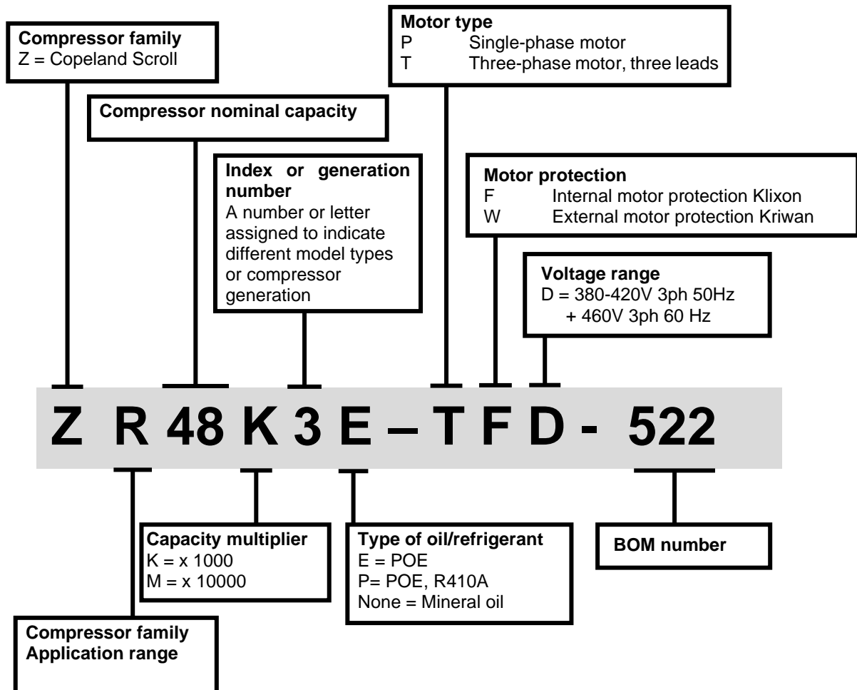
Figure 1: Example of nomenclature for a standard scroll compressor, ZR range
