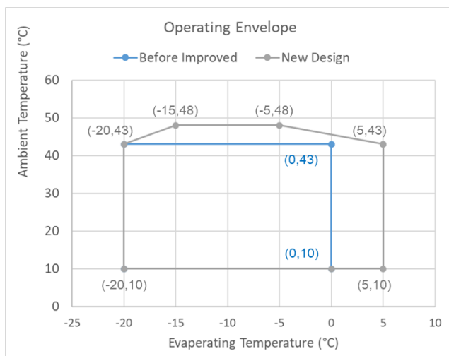
Figure 1. New ZXD091BE operating envelope
