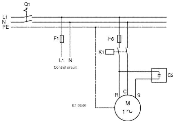
Fig. 4: Power Circuit Single-Phase
