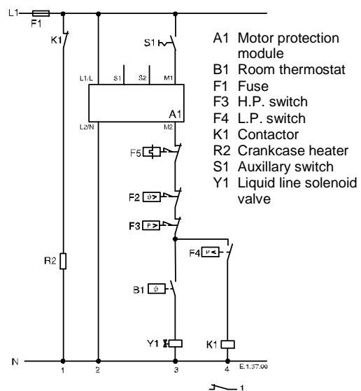
Fig. 7: Air Conditioning Scroll Control Circuit
