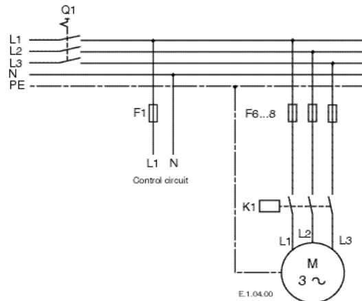
Fig. 5: Power Circuit Three-Phase
